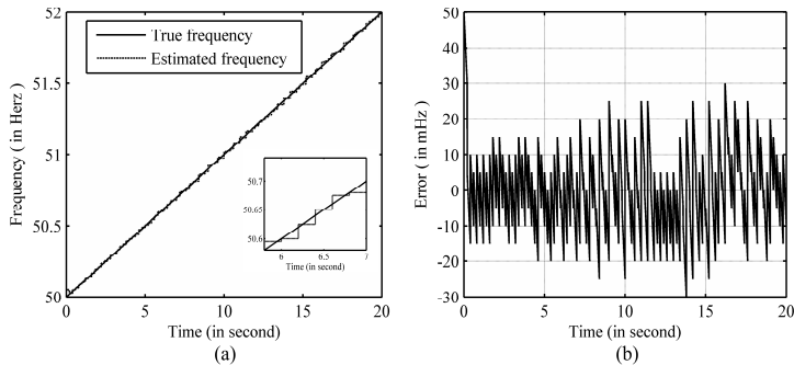
Fig. 3. Frequency tracking for ramp variation (a) frequency variation curves (b) the estimation error.
